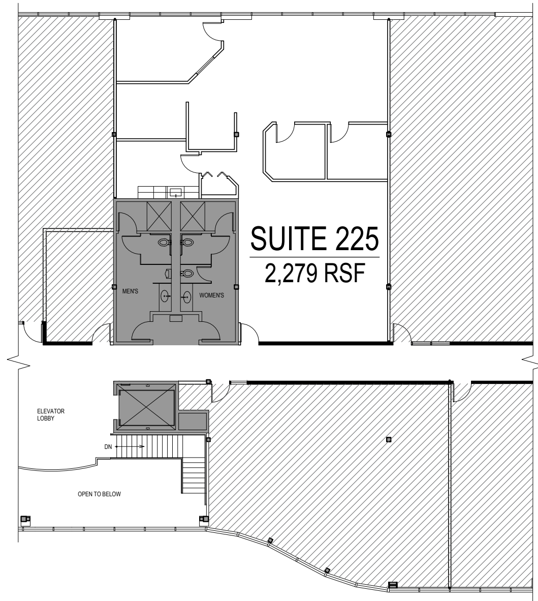
① PARTIAL SECOND FLOOR PLAN
