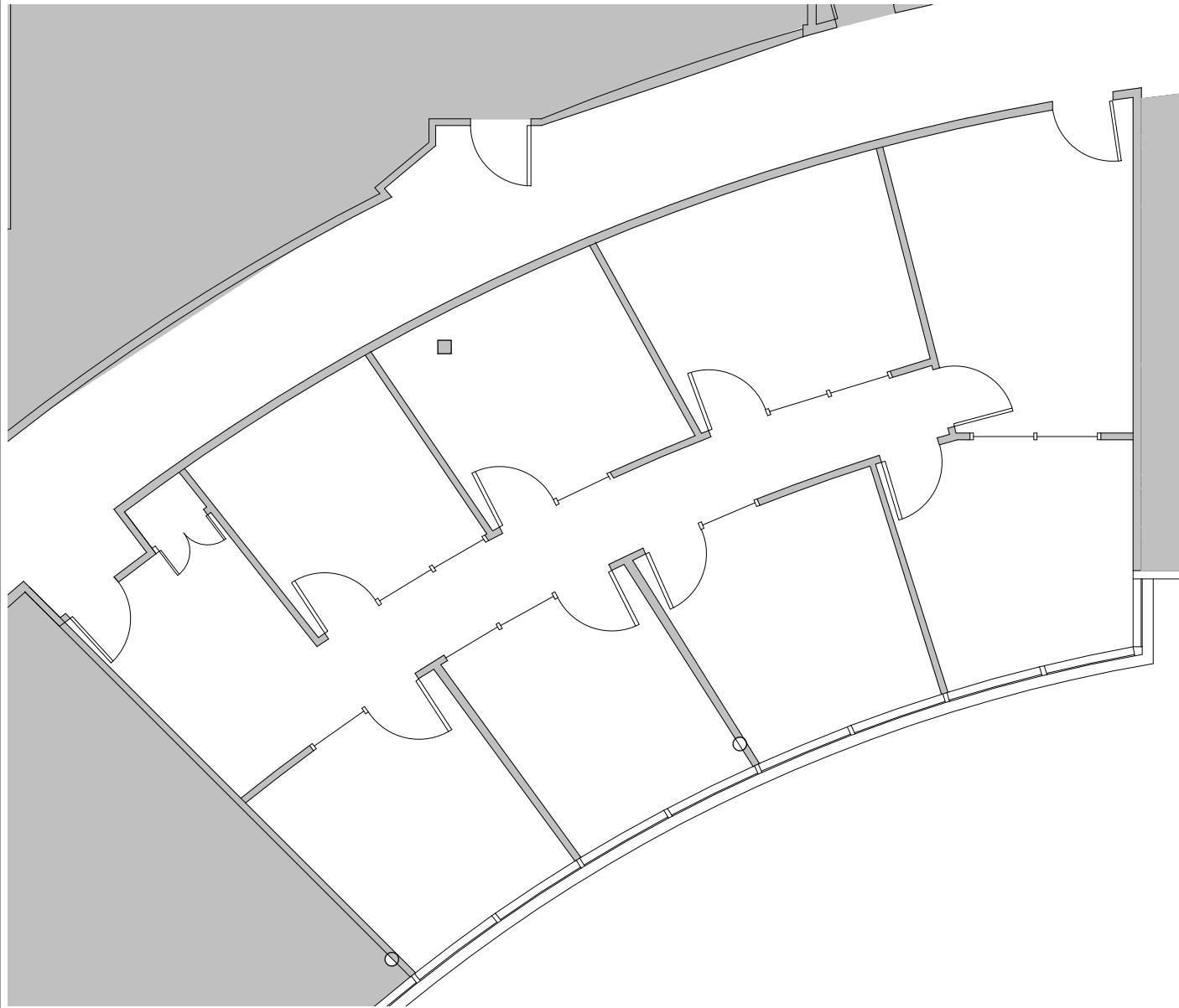
1 SUITE 1C MARKETING PLAN - 1,568 RSF 1/1 Scale: 1/8"=1'-0"
